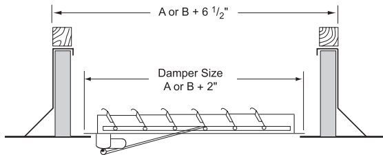
Curb for USEV/USIV and USLEV/USLIV
